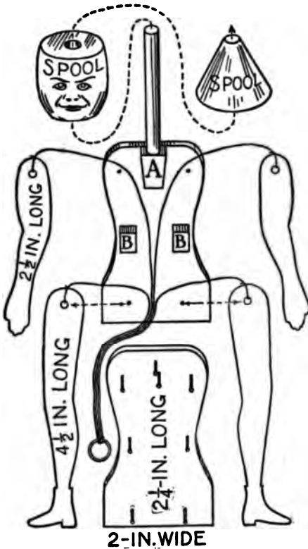
FIG. 113. — Details of Body of the Jumping-Jack shown in Fig. 110.
